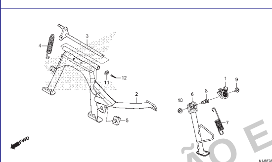
C-35 Cavalete
